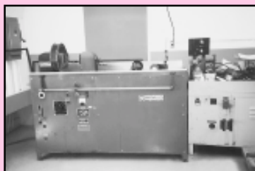
Magnaflux Machine, Type DR-523, 6' Bed, AC, 3,000 Amp Output, Single Phase
